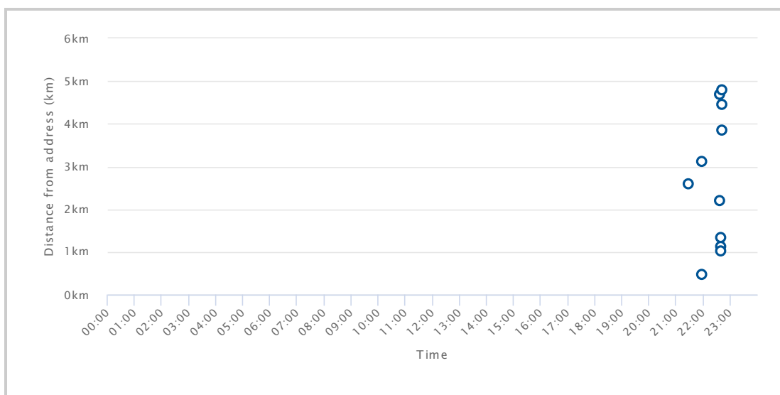
Lightning Strikes on 2018-08-08
